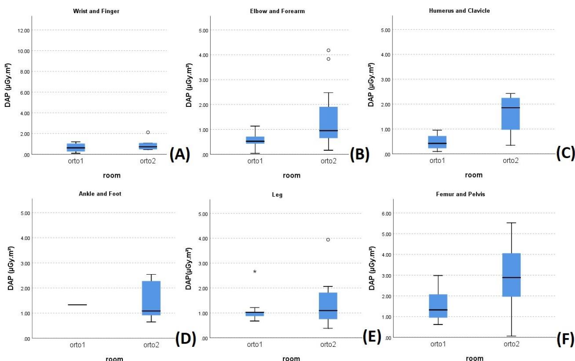
Figure 5. Mean DAP values in Orthopedic Operating Rooms 1 and 2 by surgical site. (A) to (F), respectively represent mean DAP values for imaging of the following anatomical regions: (A) Hand, (B) Elbow and forearm, (C) upper arm and shoulder, (D) Ankle and foot, (E) Leg, and (F) Femur and pelvis.
